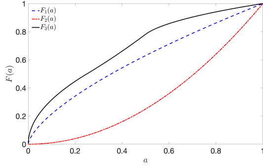
(a) CDF of Ability
