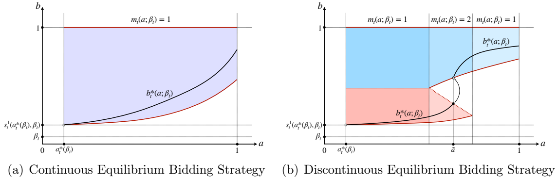
Figure 2: Illustration of Equilibrium Bidding Strategy b_t^*(a; \beta_t) .
